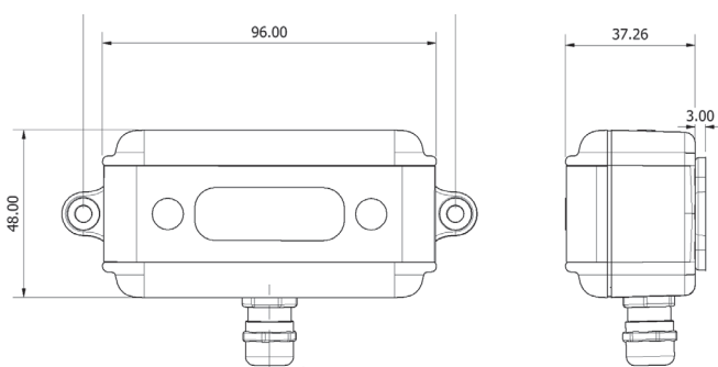
P67 cable entry
