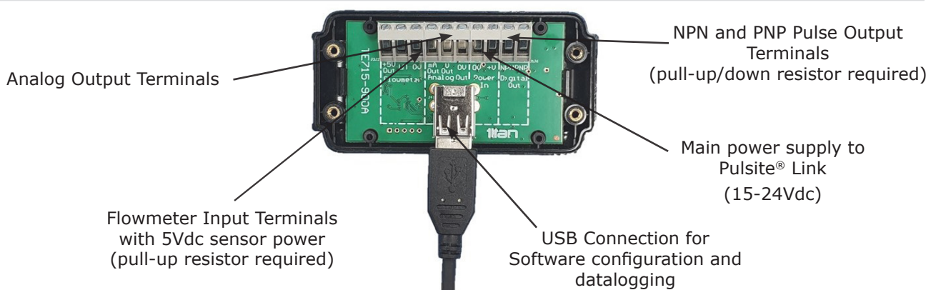
Titan's Interface Software supplied with the device allows the user to configure multiple outputs.
